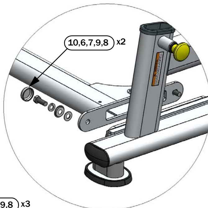
DETAIL D
