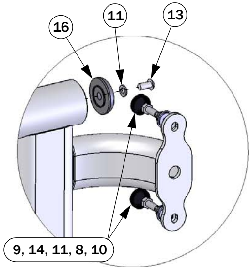
DETAIL C
