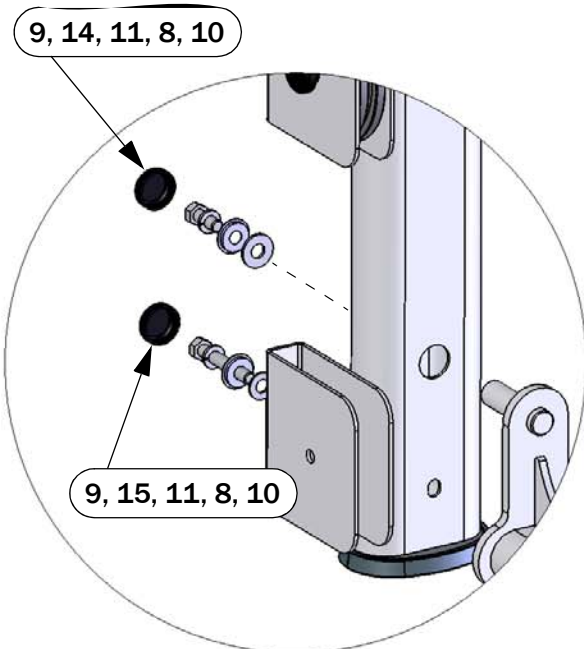
DETAIL B
